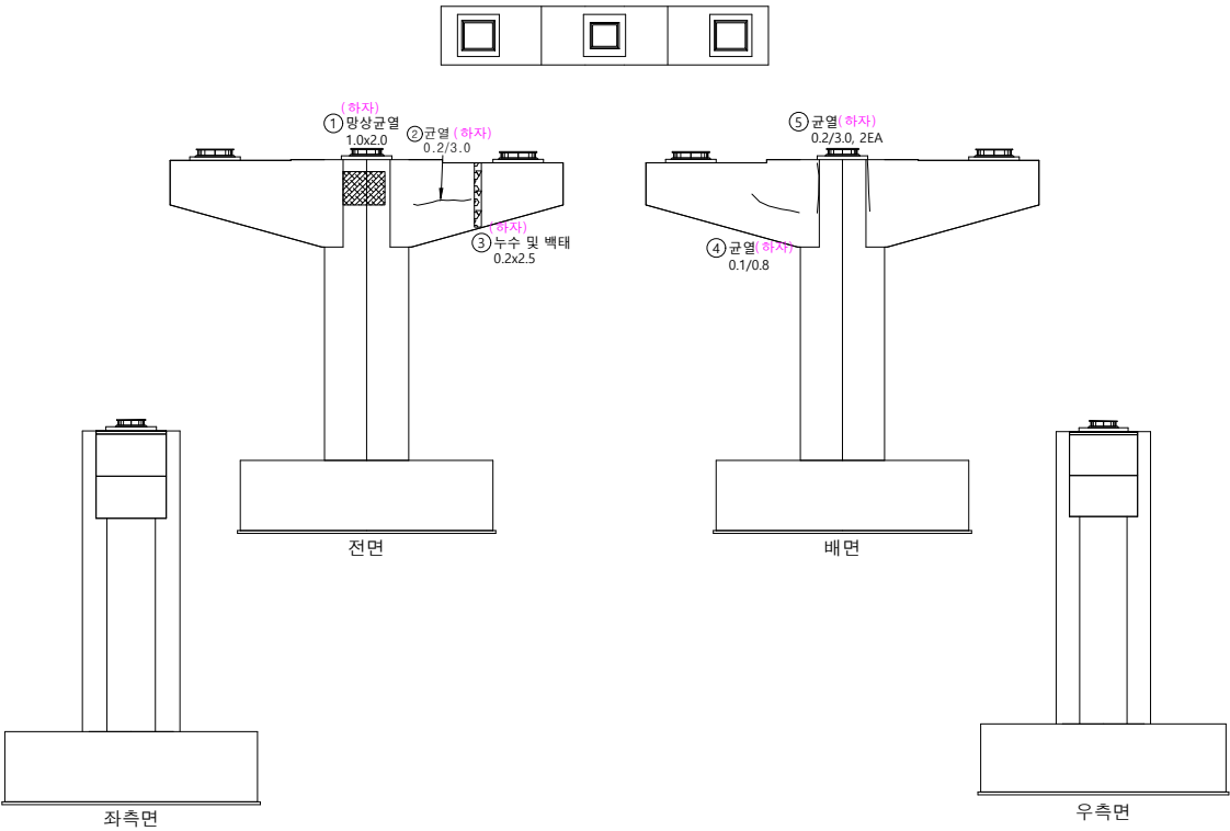
KEY PLAN
